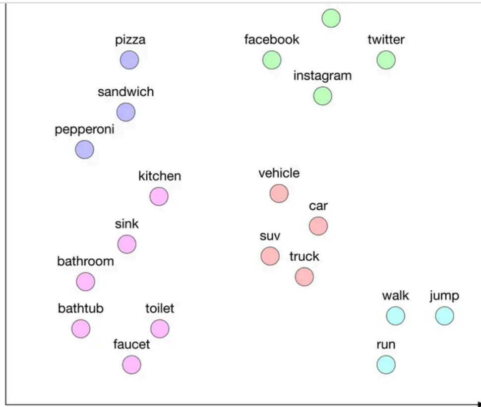
Figure 4.12: Words in the 2D embedding space
