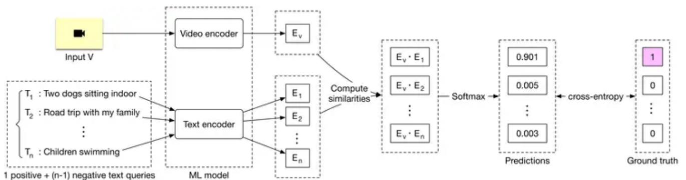
Figure 4.18: Loss computation
