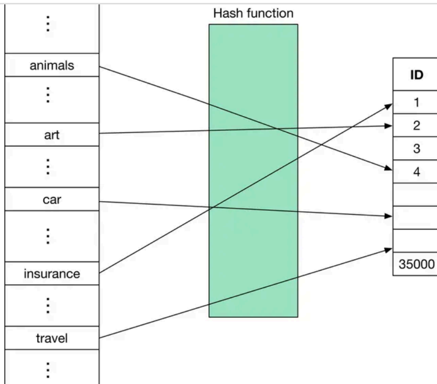
Figure 4.8: Use hashing to obtain word IDs
