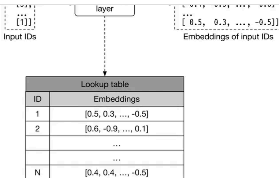
Figure 4.13: Embedding lookup method
